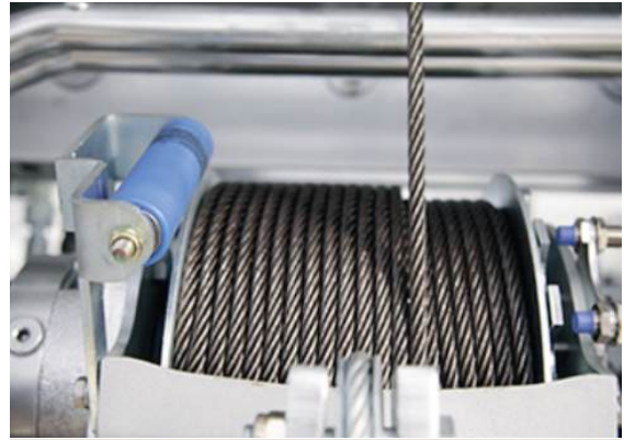
Wire detachment prevention (1 ton only)
